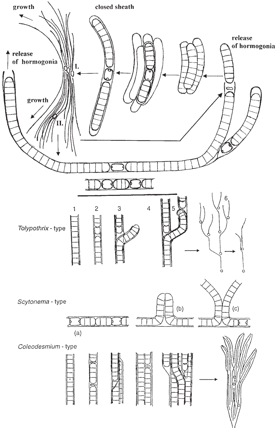
Fig. 4. – Scheme of the life-cycle of Camptylonemopsis (derived from C. sennae ) (orig.); comparison with branching type of Tolypothrix , Scytonema and Coleodesmium (from Komárek 1998).
