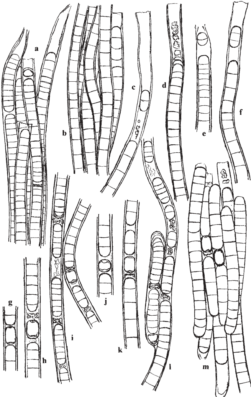
Fig. 2. – Camptylonemopsis sennae ; a – end of fasciculated filaments; b – part of fasciculated filaments; c–f – ends of filaments, partly with formation of few-celled hormogonia; g–k – parts of filaments with heterocytes, partly with fragmentation of trichomes in hormogonia; l – part of a filaments with fragmented trichome and typical coleodesmioid branching; m – fasciculated young trichomes with developing heterocytes (orig. drawing).
