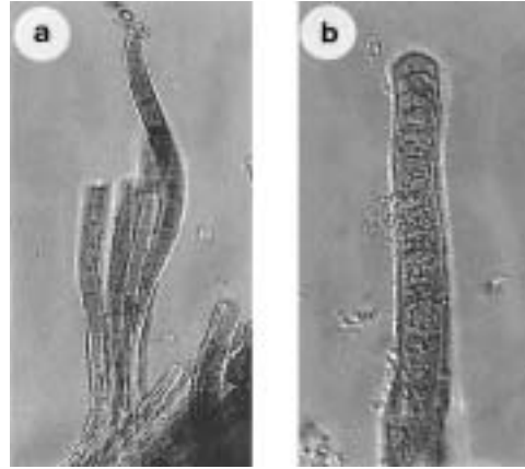
Fig. 3. – A. Camptylonemopsis sennae ; a–b – ends of fasciculated and solitary trichomes (orig. photo J. Komárková).
