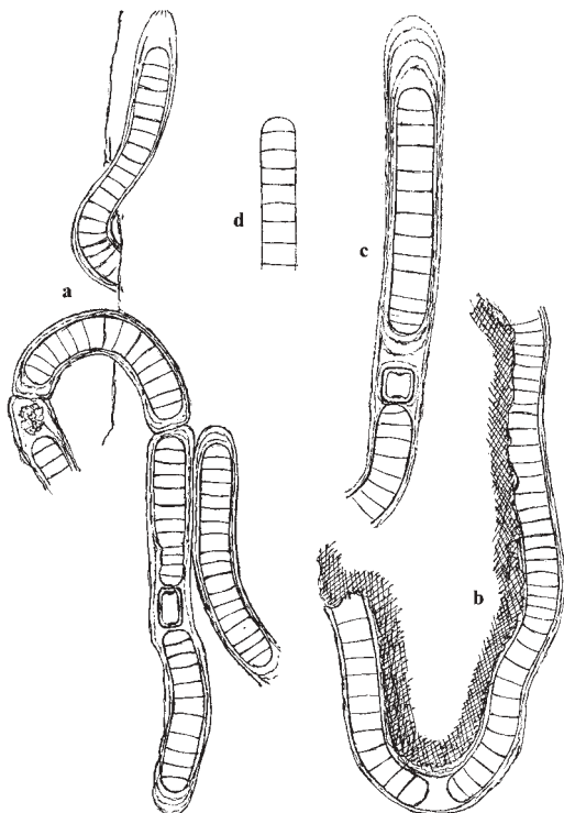
Fig. 1. – Camptylonemopsis epibryos ; a – part of creeping filaments with typical branching and one heterocyte; b – part of a creeping filament without heterocytes; c – end of filament with a heterocyte; d – end of a trichome (orig. drawing).
