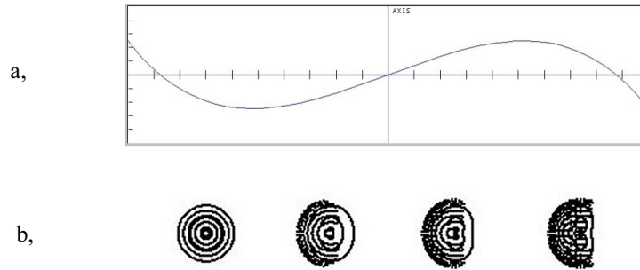
Fig.4. : The lensless Schmidt camera – a, transverse aberration ( the same for fields of view 0°- 20° ) b, spot diagrams for fields o view 0°,10°,15°,20° ( from the left ).
