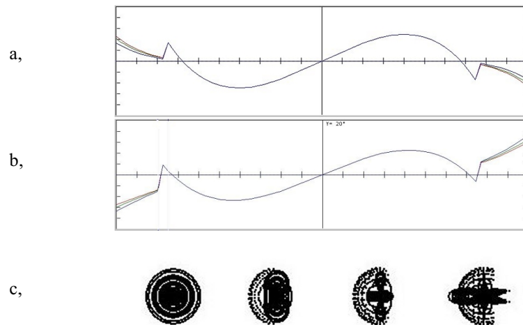
Fig.7.: The upgrade FD system a, transverse aberration for field of view 0°, b, transverse aberration for field of view 20°, c, spot diagrams for fields of view 0°,10°,15°,20° ( from the left )
