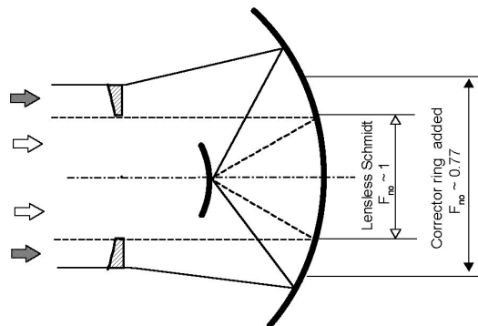
Fig. 6.: The upgrade of FD optical system - illustration
