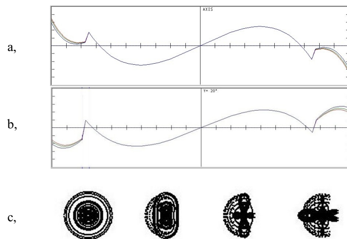
Fig.9.: The FD system with “circular arc” substitution of the aspheric corrector ring profile :
