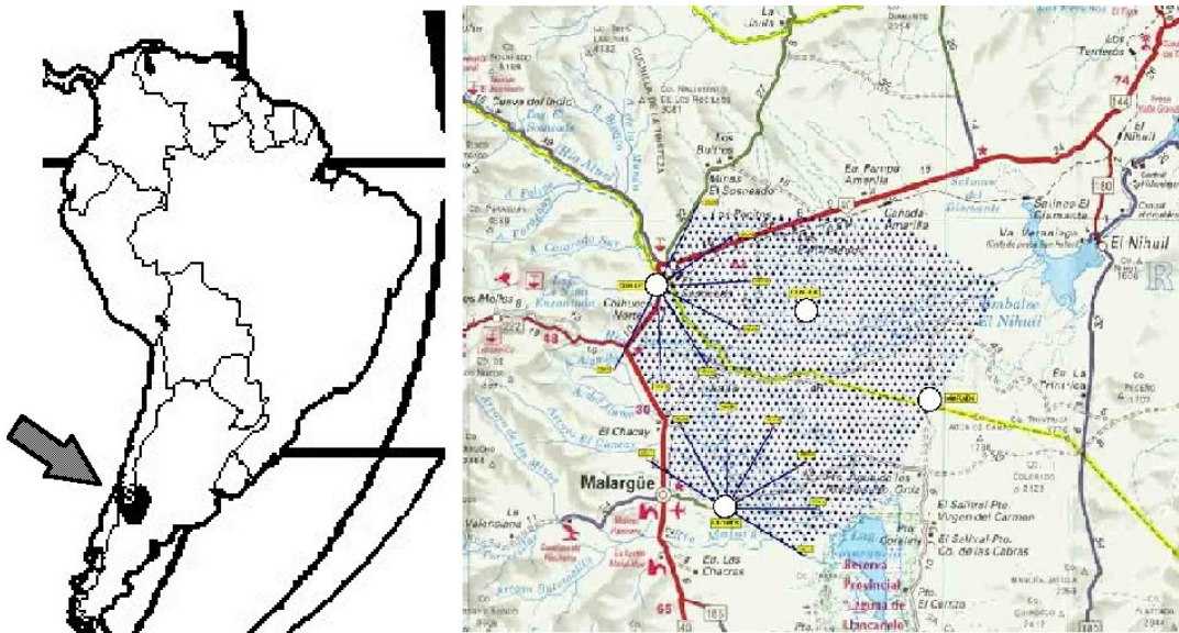
Fig.1.: The water Cerenkov detectors array and four FD planned positions.
