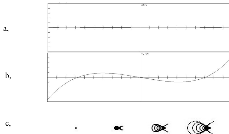
Fig.5.: The ordinary Schmidt camera – a, the transverse aberration for field of view 0°, b, the transverse aberration for field of view 20°, c, spot diagrams for fields o view 0°,10°,15°,20° ( from the left ).
