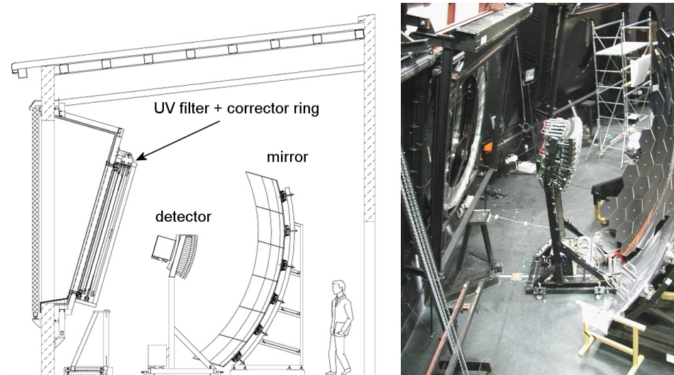
Fig. 10 . : The CAD drawing and photo of the FD prototype
