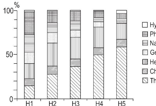
Fig. 6. – Percentage of life forms (Hy: hydrophytes, Ph: phanerophytes, Na: nanophanerophytes, Ge: geophytes, He: hemicryptophytes, Ch: chamaephytes, Th: therophytes) occurring in the habitats with varying intensity of human impact factors; for the degrees of hemeroby see Table 1.
