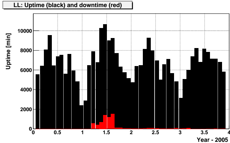
Figure 5: Uptime (black) and downtime (red) caused mainly by lidar's veto for one building of fluorescence detector. Seasonal variations of uptime are clearly visible.
