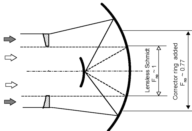
Figure1: Drawing of FD telescope optical system.
