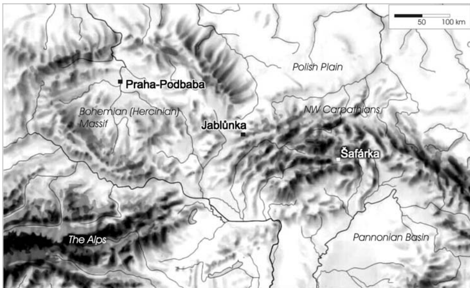
Fig. 1. – Orographic map of eastern central Europe giving the location of the sites investigated. The map includes the Czech Republic, Slovakia, Hungary, Austria, Poland and Germany.
