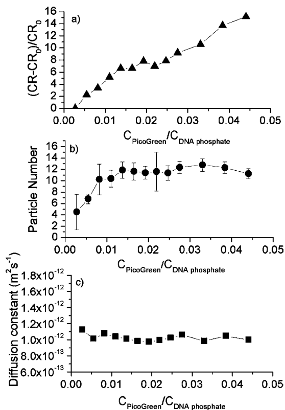
Fig. 4. Titration curve for the PicoGreen. The dependence of \beta Apr-1-Neo plasmid (10 kbp, contour length 3.4 \mu\text{m} ) diffusion constant, D_t , Particle Number, relative count rate (\text{CR} - \text{CR}_0)/\text{CR}_0 and correlation on the C_{\text{PicoGreen}}/C_{\text{DNA phosphate}} ratio.
