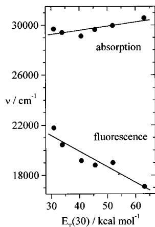
Fig. 2. Spectral positions of absorption and fluorescence maxima of DANsamide in different solvents plotted vs E_T(30) solvent polarity values ( c_{\text{DANSamide}} = 10^{-5} M ). Points correspond to experimental values in cyclohexane, toluene, dichloromethane, acetonitrile, ethanol, and water [in the order of increasing E_T(30) values]. Lines are linear fits to the experimental data.
