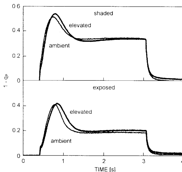
Fig. 2. Chlorophyll a fluorescence induction kinetics converted to 1 - q_p induced by actinic radiation for shaded ( upper panel ) or exposed ( lower panel ) needles from Norway spruce grown in AC ( thin line ) or EC ( thick line ). Mean of twelve curves is presented. Measurements after three years of exposure of trees to elevated CO 2 .
