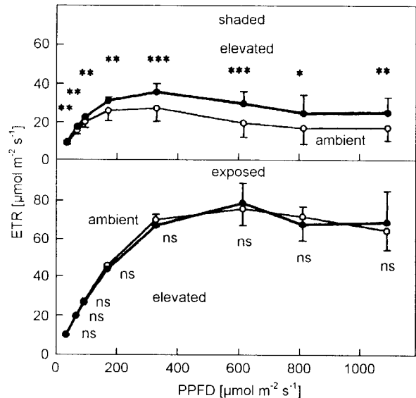
Fig. 1. The photosynthetic photon fluence density (PPFD) responses of steady state electron transport rate through PS2 (ETR) in shaded ( upper panel ) or exposed ( lower panel ) shoots grown in AC ( thin line; open circles ) or EC ( thick line; full circles ). Measurements after three years of exposure of trees to elevated CO 2 . Error bars are ± SD ( n = 12). * p = 0.05, ** p = 0.01, *** p = 0.001, ns – not significant.
