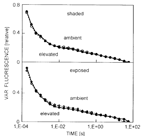
Fig. 3. Relative variable fluorescence (F - F_0)/(F_M - F_0) following an actinic flash that reduced the primary quinone acceptor Q_A in needles of Norway spruce. The open circles represent an average of 10 measurements with shaded needles treated in AC ( upper panel ); full circles – shaded needles treated in EC ( upper panel ); open diamonds – exposed needles in AC ( lower panel ); full diamonds – exposed needles in EC ( lower panel ).
