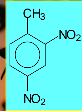
2,4-dinitrotoluene (DNT)
