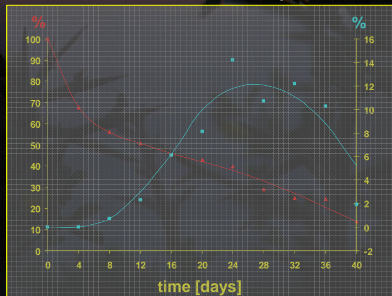
2-amino-4-nitro phenol
