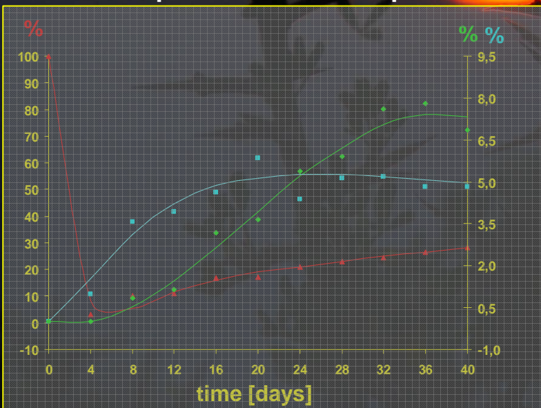
1-diazo-2-naphthol-4-sulphonic acid
