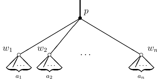
FIGURE 6. The tree defining the cup product.
