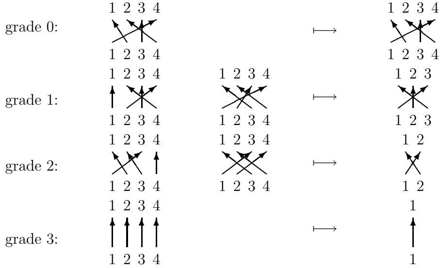
FIGURE 1. Left: Examples of elements of \Sigma_4 of grade 0 (first line), grade 1 (second line), grade 2 (third line) and grade 3 (fourth line). Right: the corresponding primitive elements.
