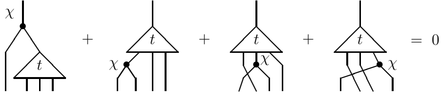
FIGURE 3. Equation (15) for n = 3 .
