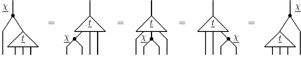
FIGURE 4. Equation (18) for n = 3 .
