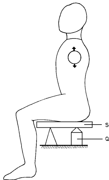
Fig. 1. Scheme of portable quantitative ballistocardiograph. S – seat, Q – piezoelectric transducer.
