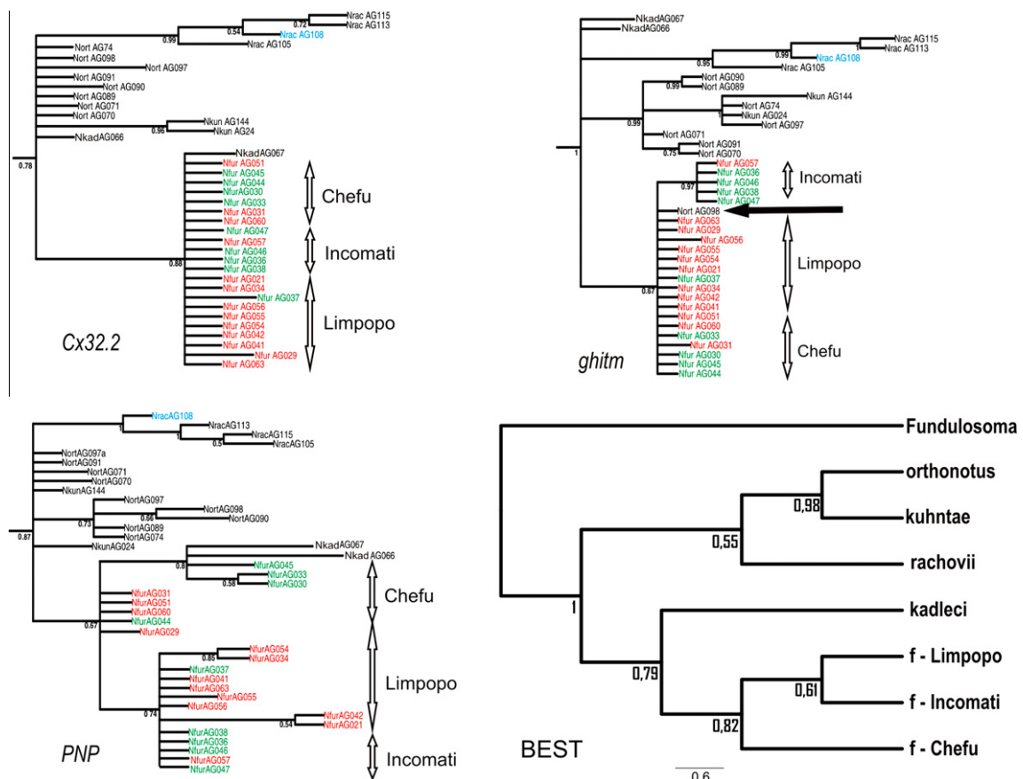
Fig. 2. Phylogenetic relationships among Nothobranchius specimens reconstructed by MrBayes, using gene trees for CX32.2 , ghitm and PNP ; and the species tree obtained using the BEST approach. Bayesian posterior probabilities (only BPP > 0.50) for nodal support are shown. In each gene tree, the morphs of N. furzeri are indicated by red (red morph) and green (yellow morph) text and N. rachovii sensu stricto by blue text. The geographical origin of N. furzeri specimens is indicated with vertical lines. The black arrow in the GHITM gene phylogram indicates a N. orthonotus specimen that clustered with N. furzeri . The BEST species tree was based on 40 specimens sequenced for all loci; with N. furzeri specimens being split according to their geographical origin (Limpopo, Incomati and Chefu) in order to test the robustness of drainage divisions (see Methods for more details).
