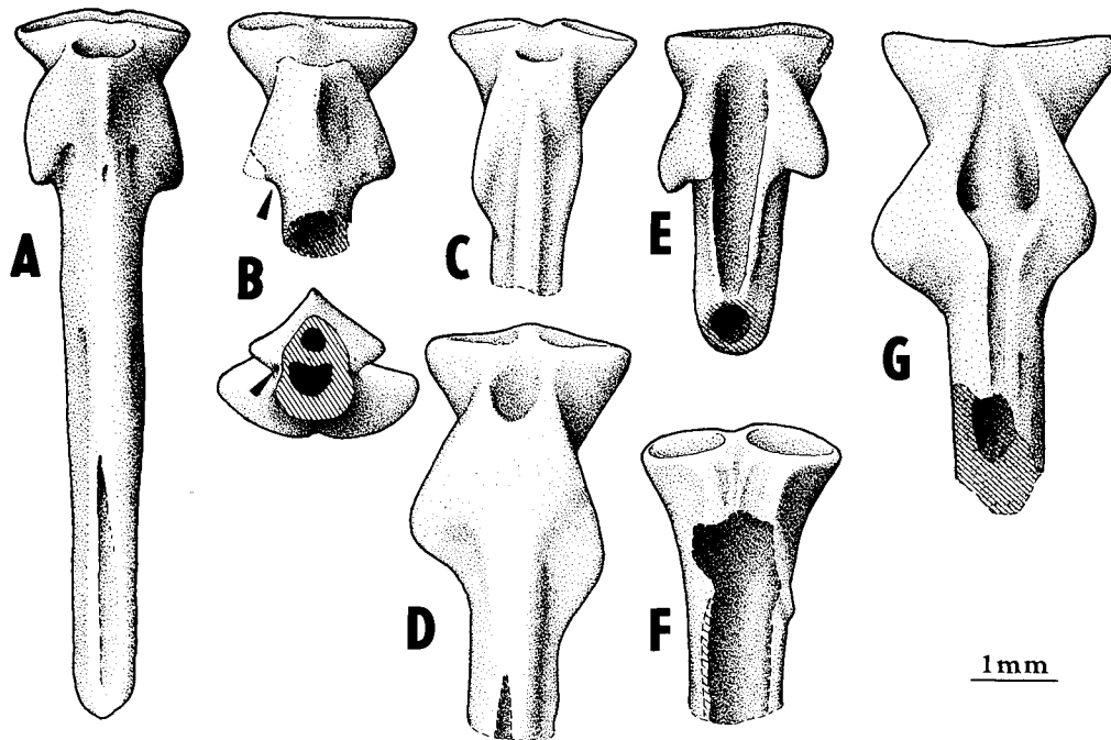
Text-fig. 17. Gobiatidae indet. or Discoglossidae indet. Urostyles in dorsal view. A - LU-N 5/243. B - LU-N 5/213 (see also Pl. 4, fig. 7; below is the same specimen in posterior view, to show position of the intervertebral canal which is marked by an arrow). C - LU-N 3/46. D - LU-N 6/404. E - LU-N 5/205. F - LU-N 2/8. G - LU-N 6/395 (see also Pl. 4, fig. 8).
