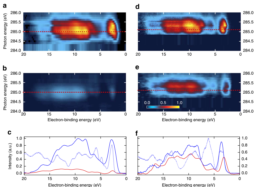
Figure 4 | Resonant photoemission results. Resonant photoemission (RPES) intensity map of LUMO and LUMO +1 resonances of multilayer (a) and monolayer (b) of 22PCP. (c) Line profiles of LUMO resonances for monolayer (red) and multilayer (blue) 22PCP with the valence band spectrum (dashed blue, 140 eV photon energy). The corresponding panels for 44PCP are shown in d,e and f. The intensities of both valence band spectra have been scaled for clarity.
