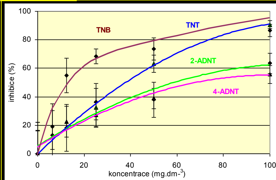
TNT 100mg/l
