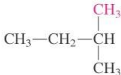
2-Methylbutane (Isopentane)
