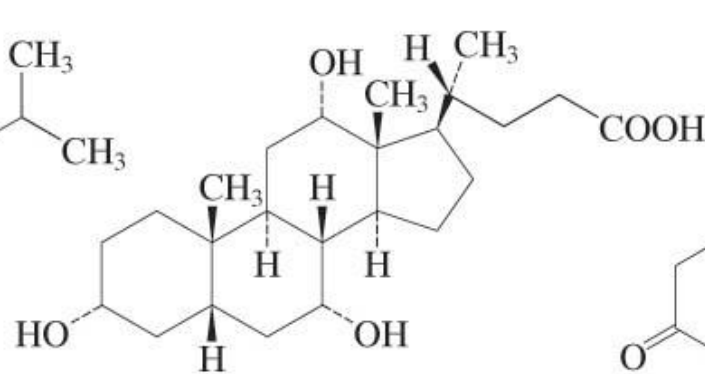
Cholic acid
