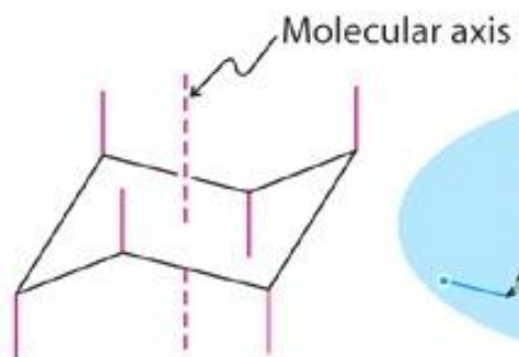
Axial positions
