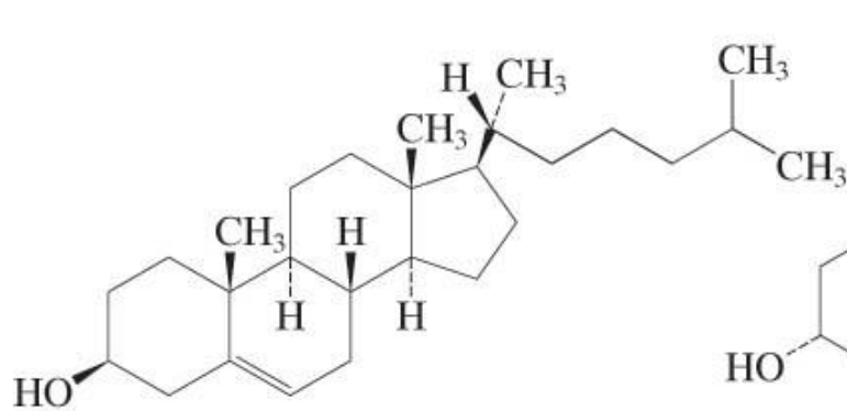
Cholesterol
