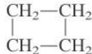
Cyclobutane, \text{C}_4\text{H}_8
