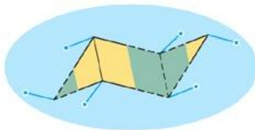
Equatorial positions
