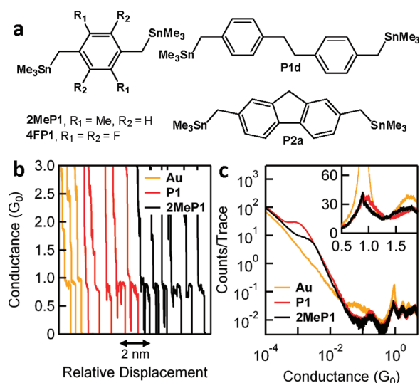
Figure 3. (a) Structures of additional compounds studied. (b) Individual conductance traces measured in solutions of the \text{SnMe}_3 -terminated compounds P1 (red) and 2MeP1 (black) at 25 mV applied bias. (c) Conductance histograms of over 10 000 individual measurements, generated with linear bin size of 0.0001 G_0 , shown on a log–log scale. Inset: same histograms on a linear scale.
