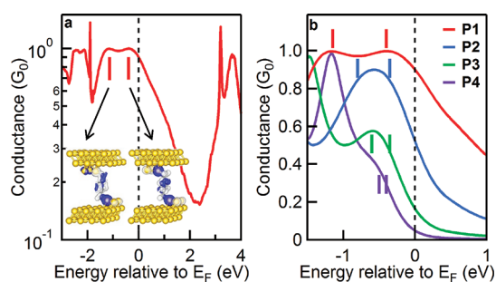
Figure 4. (a) Calculated transmission spectrum for P1 bonded to Au electrodes. Inset: isosurface plots of the real part of the transmitted scattering states for energies at the vertical bars ( -1.15 and -0.4 eV), showing the even and odd combinations of the Au–C bonds coupled through the \pi backbone. (b) Transmission spectra for P1–P4 . Bars indicate the approximate position Au–C MO energies.
