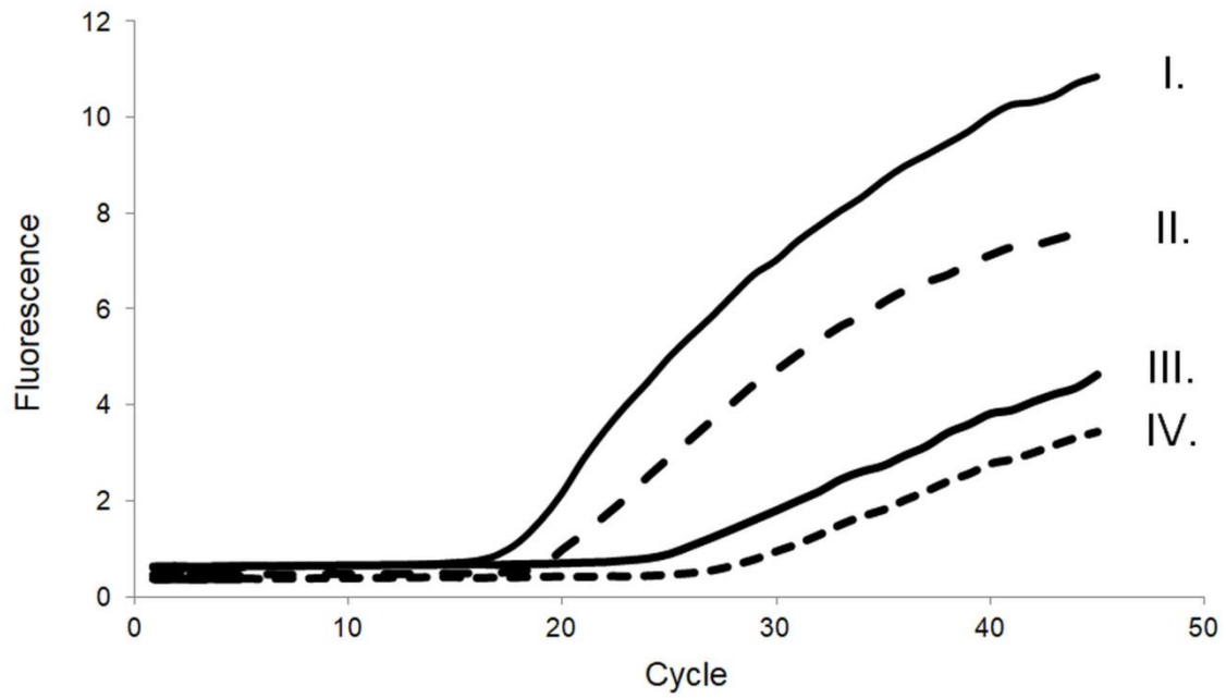
Figure 2. Lines I and II show amplification curves for wild-type (solid line) and mutant (broken line) alleles in a DNA extract from a heterozygous subject carrying Leiden mutation. Line III and IV demonstrate amplifiability of DNA present in a modified blood sample of the same subject.
