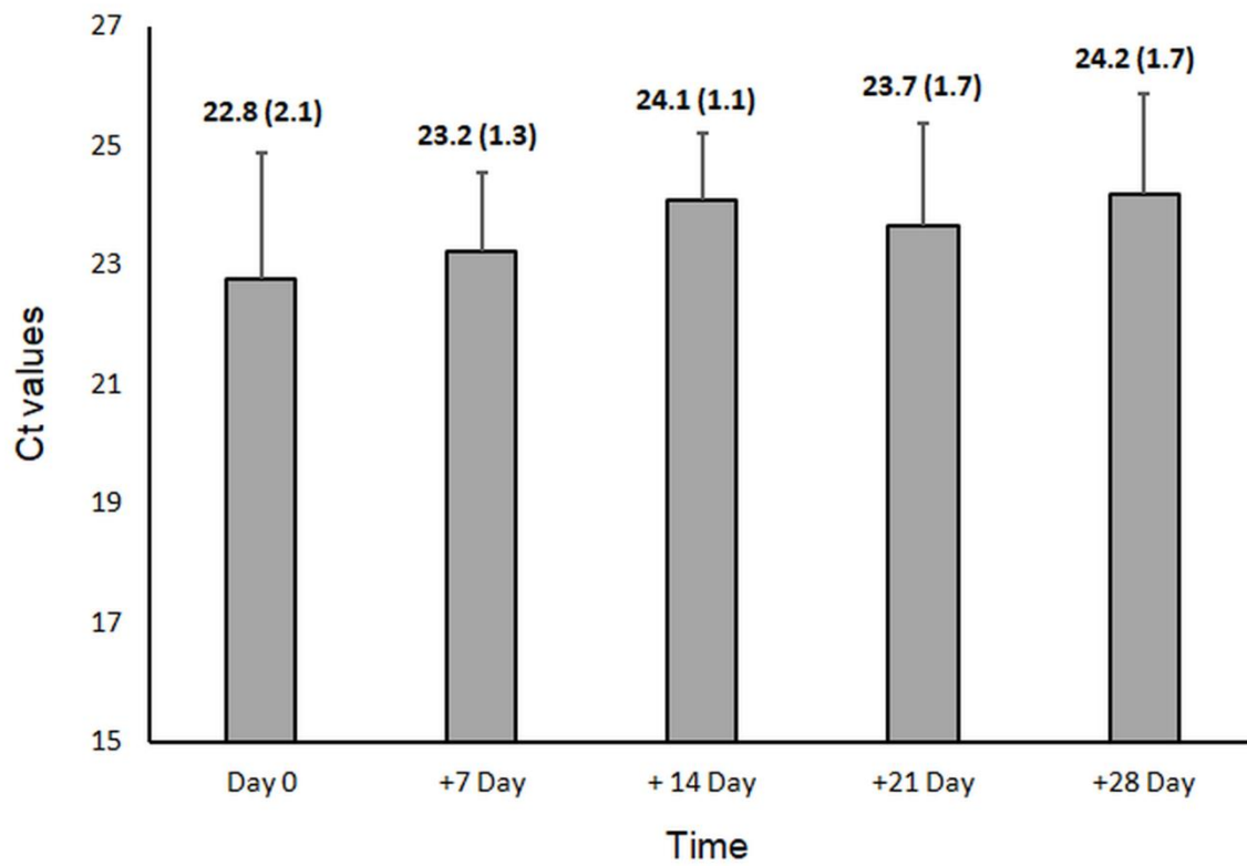
Figure 3. Stability of DNA molecules in whole blood during 28 days freezing interrupted by four cycles of thawing.
