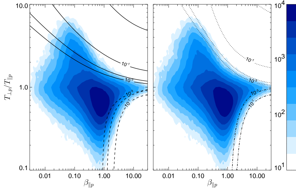
Figure 1. Both panels show a color scale plot of the relative frequency of (\beta_{\parallel p}, T_{\perp p}/T_{\parallel p}) in the WIND/SWE data (1995–2001) for the solar wind with v_{sw} \leq 600 km/s [cf. Kasper et al. , 2002, Figure 2]. The (logarithmic) color scale is shown on the right. The overplotted curves show the contours of the maximum growth rate (in units of \omega_{cp} ) in the corresponding bi-Maxwellian plasma (left) for the proton cyclotron instability (solid curves) and the parallel fire hose (dashed curves) and (right) for the mirror instability (dotted curves) and the oblique fire hose (dash-dotted curves).
