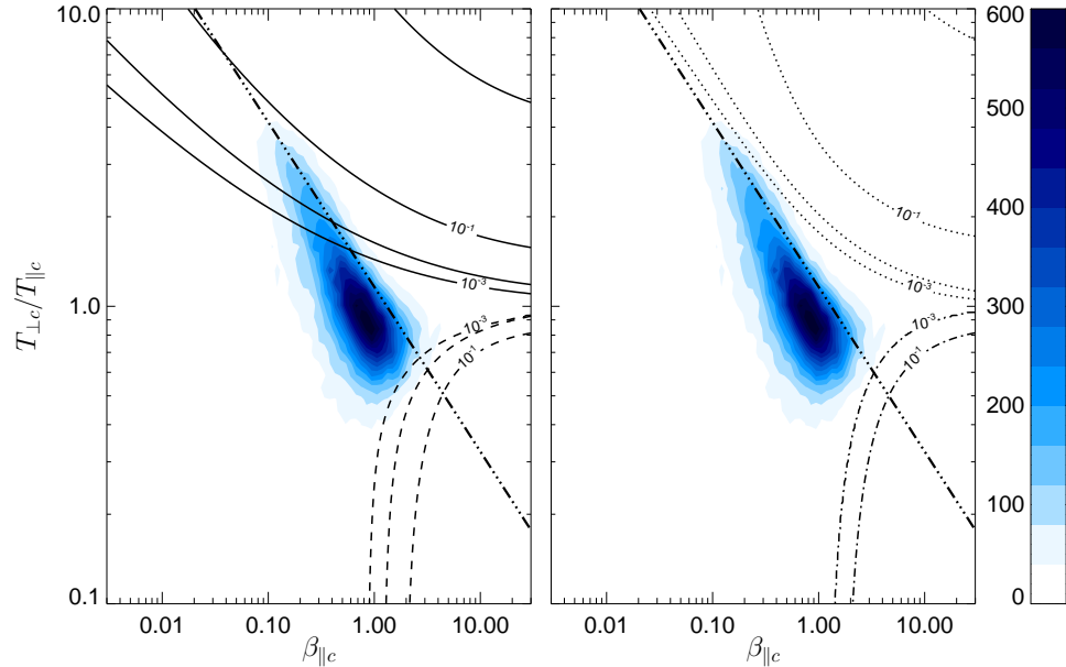
Figure 2. Both panels show a color scale plot of the relative frequency of (\beta_{\parallel c}, T_{\perp c}/T_{\parallel c}) in the WIND/SWE data (1995–2001) for the solar wind with v_{sw} > 600 km/s. The color scale is shown on the right. The overplotted curves show the contours of the maximum growth rate (in units of \omega_{cp} ) in the corresponding plasma (left) for the proton cyclotron instability (solid curves) and the parallel fire hose (dashed curves) and (right) for the mirror instability (dotted curves) and the oblique fire hose (dash-dotted curves). The dash-dot-dot-dotted lines denote equation (2) between T_{\perp c}/T_{\parallel c} and \beta_{\parallel c} found in the HELIOS data [Marsch et al. , 2004].
