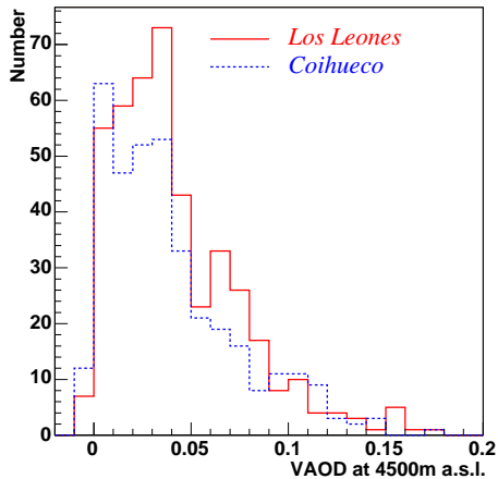
Figure 1. The distribution of VAOD from FD level to 4500m above sea level (a.s.l) reconstructed from CLF laser shots (January 2004 - February 2005). As described in the text, the VAOD measured at different FDs is expected to be slightly different.
