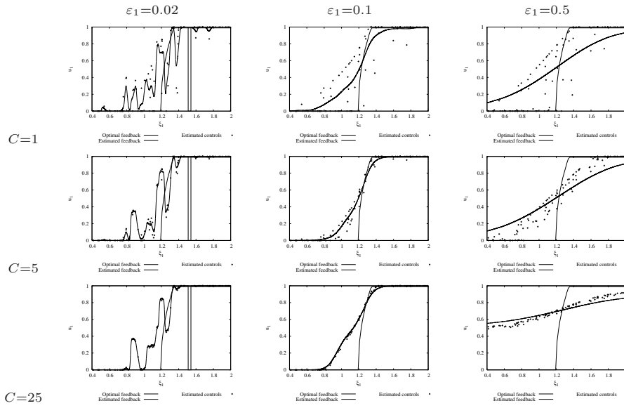
Fig. 1. Approximation of u_1(\cdot) for N = 100 scenarios as a function of the bandwidth \varepsilon_1 and the penalty C .
