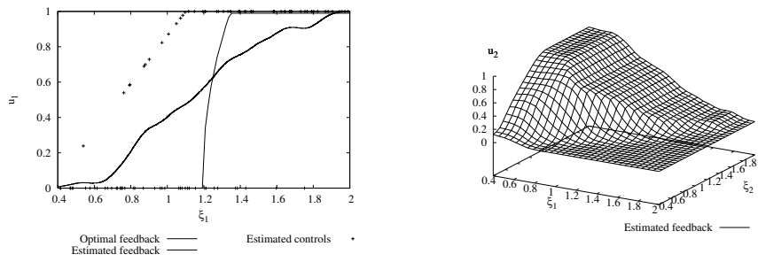
Fig. 3. Approximations of u_1(\cdot) and u_2(\cdot, \cdot) , for N = 100 scenarios, with bandwidth \varepsilon_1 = 0.1 and no penalty, i. e., C = 0 .
