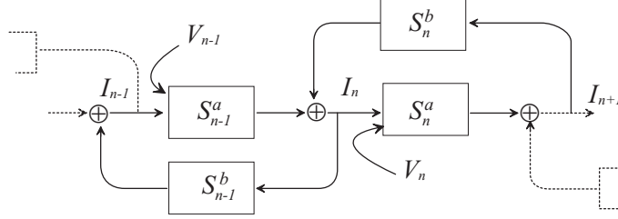
Fig. 5. Model concatenation.
