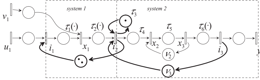
Fig. 6. TEG modeling two elementary systems concatenated.
