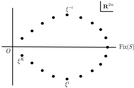
Fig. 1. Numerical homoclinic solution.
