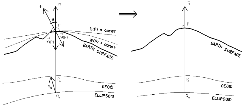
Fig. 1. Gravity and normal gravity vectors, deflection of vertical.
