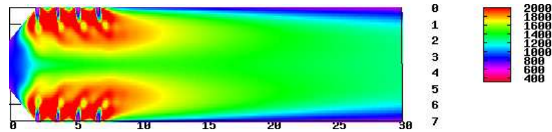
Fig. 5. Temperature profile – flue gas flow rate: 48 kg/s.
