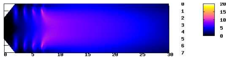
Fig. 7. Velocity profile – flue gas flow rate: 48 kg/s.
