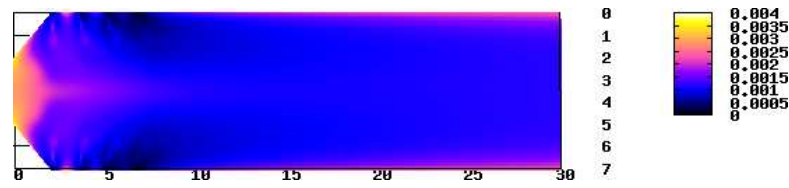
Fig. 6. NOx profile – flue gas flow rate: 48 kg/s.
