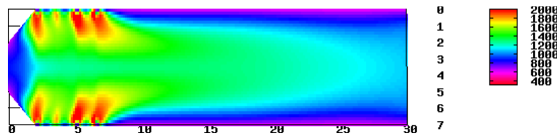
Fig. 2. Temperature profile – symmetrical channel 30 \times 7\text{m} , 2 \times 4 burners, flue gas flow rate: 18 \text{ kg/s} .
