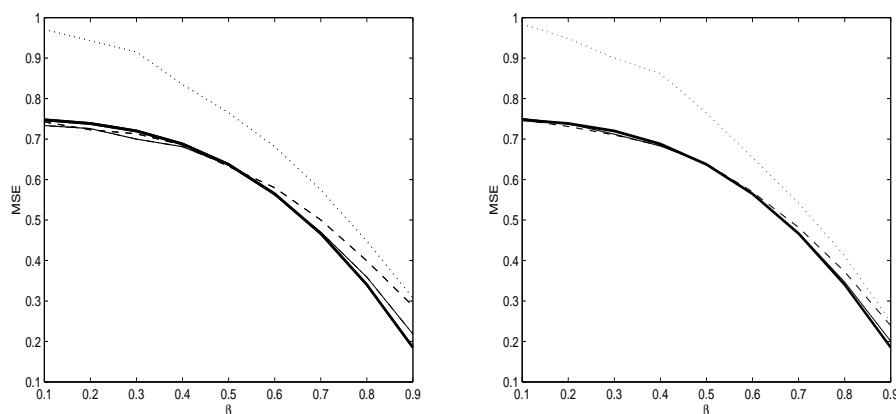
Fig. Estimates of the asymptotic mean square error of \hat{\beta} by bootstrap for n = 100 (left panel) and n = 200 observations (right panel).
