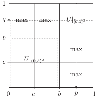
Fig. 6. Operation U \in \mathcal{U}(e) continuous in the open unit square with b < 1 .
