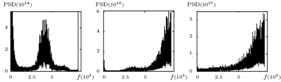
Fig. 3. (a) \beta = 1.25, \mu = 2.25 (b) \beta = 1.55, \mu = 2.25 (c) \beta = 1.99, \mu = 3.0 .
