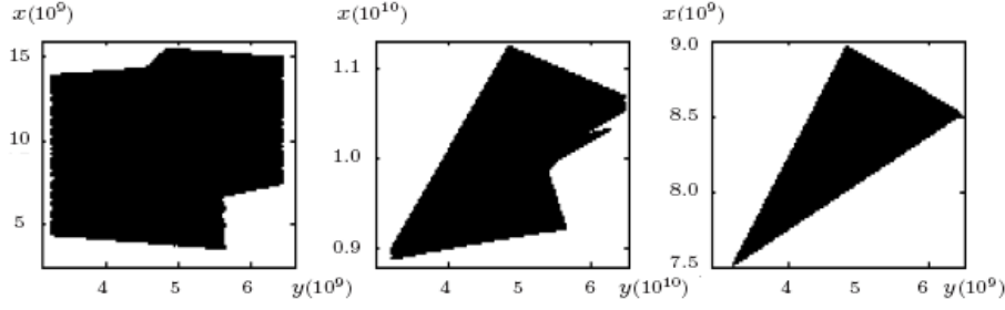
Fig. 4. (a) \beta = 1.5, \mu = 3.99 (b) \beta = 1.5, \mu = 3.0 (c) \beta = 1.5, \mu = 2.5 .
