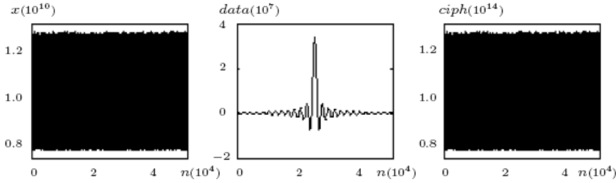
Fig. 5. (a) N -Logistic-tent (b) data (c) ciphertext.
