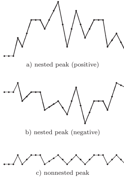
Fig. 1. Examples of waveforms with the same structural description 00pnpp00npppnppnnpp00nppnn.
