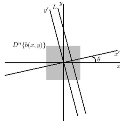
Fig. 6. Radon transformation.
