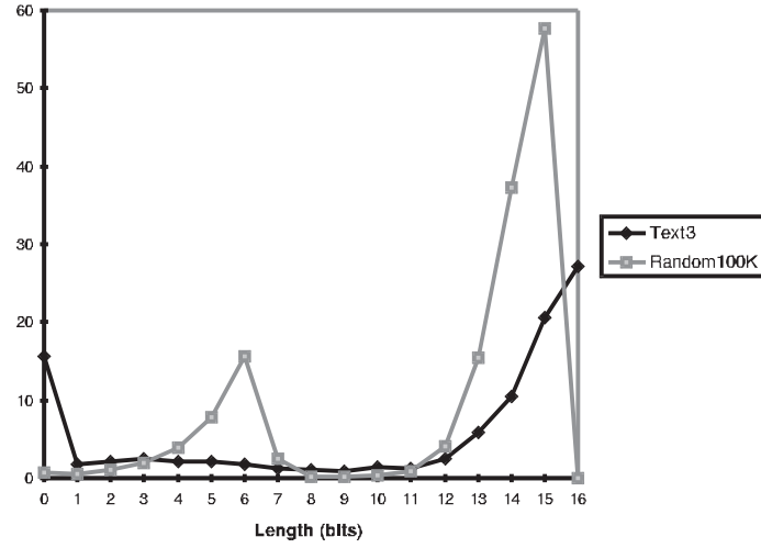
Fig. 6. Edge Length Distribution (Length – bits, # of edges in percent).
