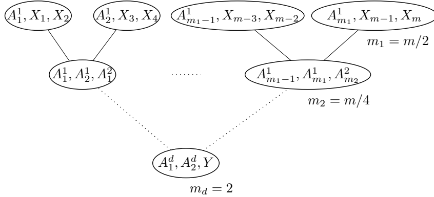
Fig. 3. Junction tree for the parent divorcing method.
