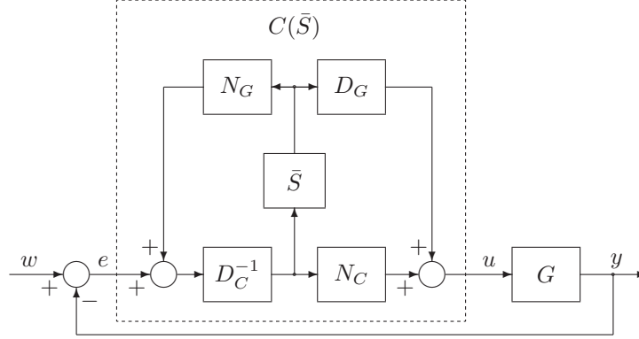
Fig. 2. Block diagram of the closed-loop system.
