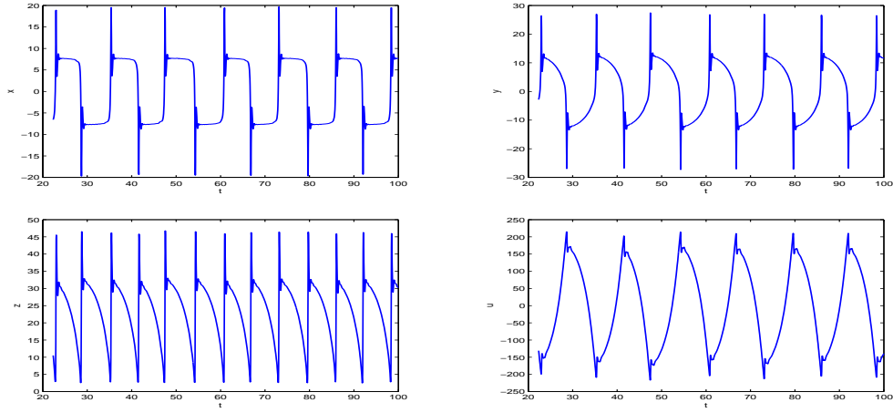
Fig. 3. When k_1 = -10.1 , k_2 = -2.2 , \tau_{10} = 0.09 , \tau_{20} = 0.99 , the time response of the controlled hyperchaotic Lü system.
