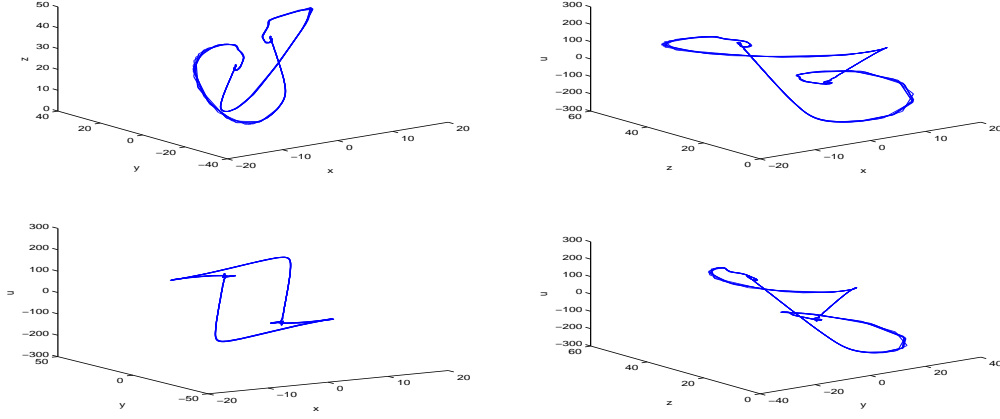
Fig. 2. When k_1 = -10.1 , k_2 = -2.2 , \tau_{10} = 0.09 , \tau_{20} = 0.99 , the state trajectories of the controlled hyperchaotic Lü system.
