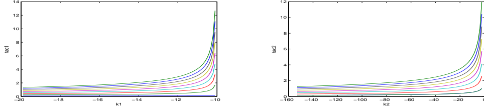
Fig. 1. When k_1 \in [-19.9, -10.1] , k = 0, 1, \dots, 8 , the graphs show the relationship between the parameters k_1 and \tau_{1k}, k_2 and \tau_{2k} respectively.
