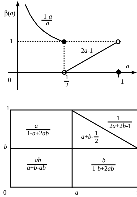
Fig. 2. Bijection \beta(a) (up) and Table 1 describing B_{\text{and}} for a, b \in (0, 1) (down).
