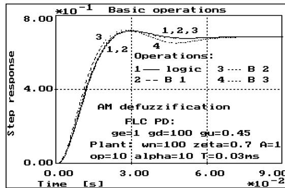
Fig. 4. Example of results for fuzzy PD control.
