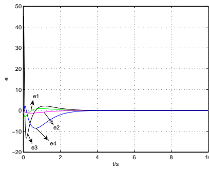
Fig. 9. The GS error curve of the hyperchaotic system when velocity is improved.
