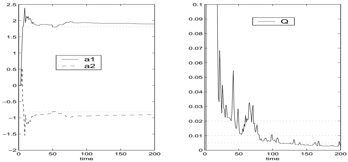
Figure 2. Left: trajectories of point estimates of auto-regression coefficients. Right: the trajectory of the test statistic Q(d(t)) .
