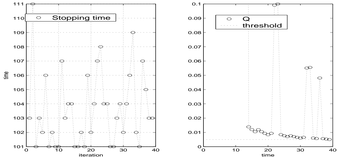
Figure 5. Independent realizations of stopping moments and the trajectory of the test statistic
