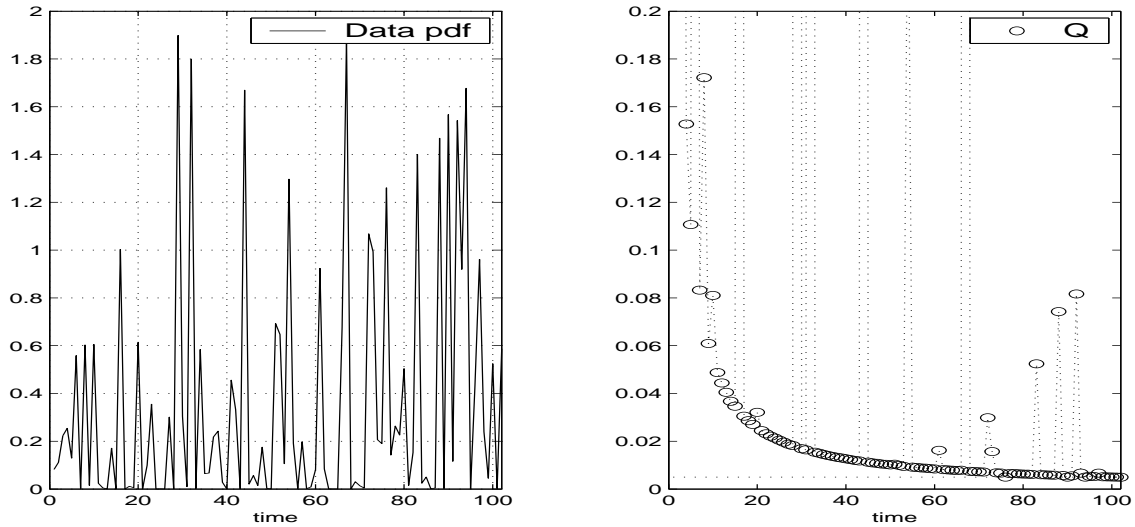
Figure 4. Trajectories of posterior data likelihood and test statistic
