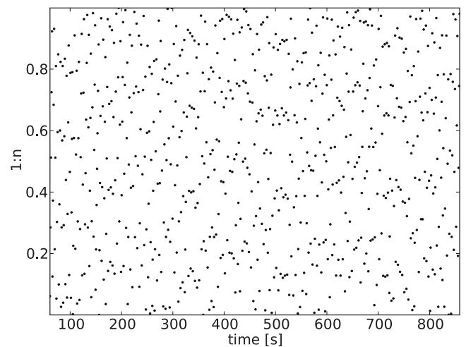
FIG. 5. Synchrogram (1:n) of the cardiorespiratory activity of the subject in the awake state.
