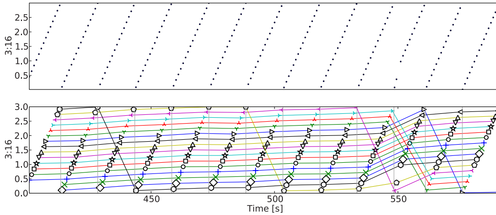
FIG. 11. (Color online) Plot of the evolution of the sequences of every 16th heartbeat of the anesthetized patient in the same coordinates as a standard synchrogram plot (synchrogram is an excerpt from nonsynchronized segment cf. Fig. 7). The fluctuations are very small and a drift toward the top of the synchrogram can be seen.
