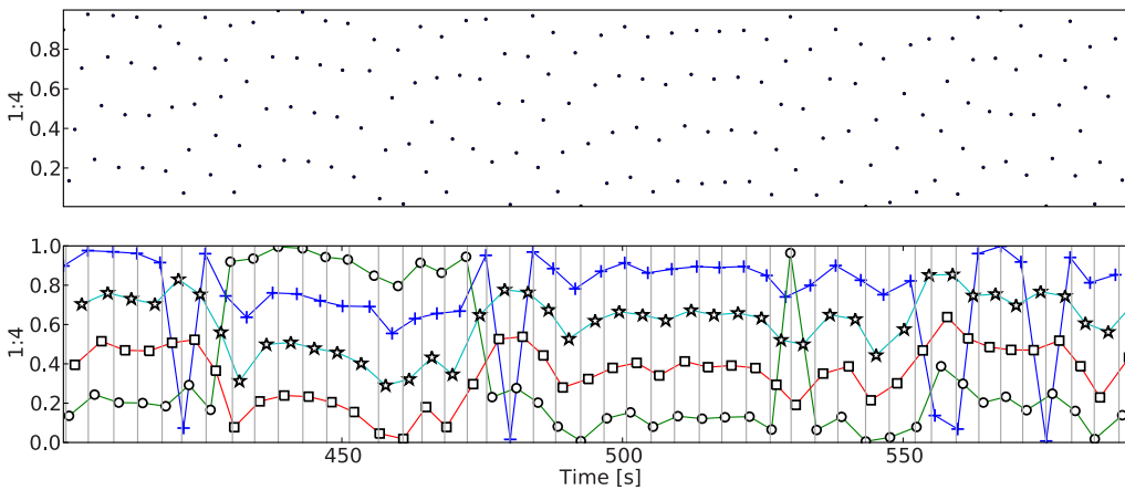
FIG. 12. (Color online) Plot of the evolution of sequences of every fourth heartbeat of the awake patient in the same coordinates as a standard synchrogram plot (synchrogram is excerpt from synchronized region in Fig. 5). There is no apparent drift of the sequences but large fluctuations can be seen.
