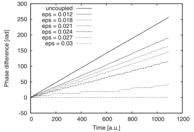
FIG. 1. Evolution of the phase differences for different strengths of coupling C from a pair of symmetrically coupled Rössler oscillators (9).
