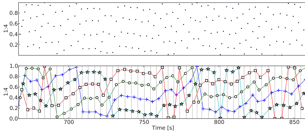
FIG. 13. (Color online) Plot of the evolution of sequences of every fourth heartbeat of the awake patient in the same coordinates as a standard synchrogram plot (synchrogram is an excerpt from nonsynchronized segment cf. Fig. 5). The sequences clearly drift toward the top, even though the fluctuations are large.
