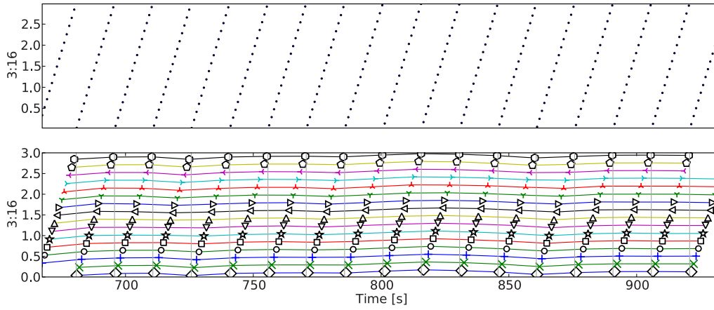
FIG. 10. (Color online) Plot of the evolution of the sequences of every 16th heartbeat of the anesthetized patient in the same coordinates as a standard synchrogram plot (synchrogram is an excerpt from synchronized segment, cf. Fig. 7). The fluctuations are very small and there is no apparent drift of the sequences.
