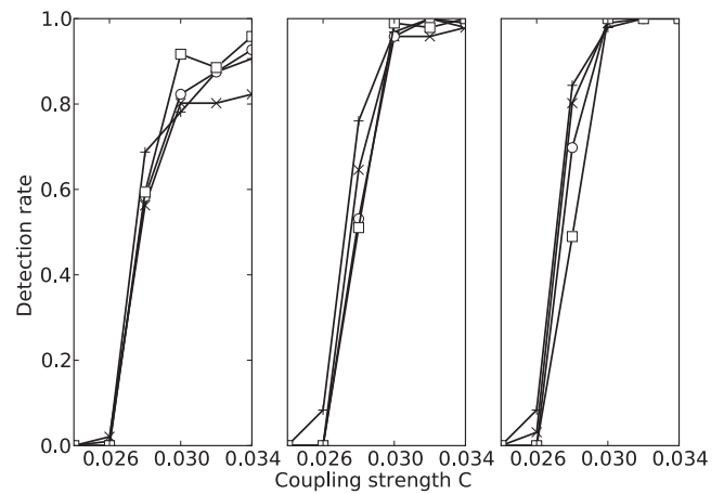
FIG. 3. Results of the proposed method for symmetrically coupled Rössler oscillators: detection rates for least trimmed squares estimation with h = N/2 + 1 (left), h = \frac{3}{4}N (center), and ordinary least-squares estimation, h = N (right). Epoch lengths: 34 periods (pluses), 68 periods (crosses), 136 periods (circles), and 273 periods (squares).
