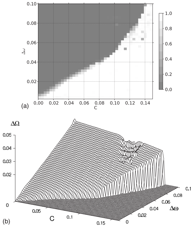
FIG. 2. Detection rates for the proposed method using least trimmed squares ( h = \frac{3}{4}N ) from short time series of \approx 18 periods (a) and difference of mean frequencies for a symmetrically coupled Rössler system pair (b) from Ref. 14, used with permission. C represents the coupling strength, \Delta\omega represents the nominal frequency mismatch and \Delta\Omega is the actual frequency difference computed from the time series. The systems are considered synchronized when the computed frequency difference \Delta\Omega is negligible. In this region, the detection rates are close to 1 almost everywhere.
