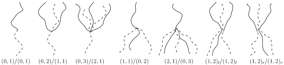
FIG. 6. Types of points in the Brownian web and its dual (\mathcal{W}, \hat{\mathcal{W}}) .
