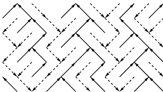
FIG. 4. Dual arrow configuration with no branching.
