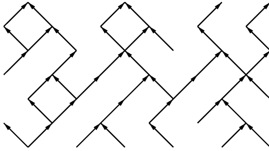
FIG. 1. An arrow configuration.
