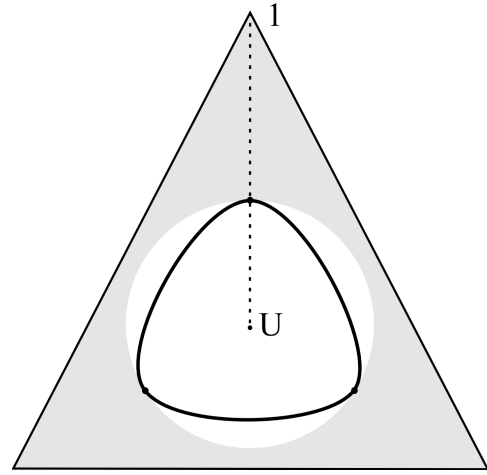
Fig. 3. In the simplex of distributions on a 3-element set, the distributions with index of coincidence less a certain value are indicated by the shaded area. A level curve of the entropy function is indicated by a full curve. Mixtures of the uniform distribution U and a Dirac distribution at one of the extreme points is indicated by a dashed line. Maximal entropy over the shaded area is obtained at the point where the dashed line leaves the shaded area. The two other points with maximal entropy are indicated as well.
