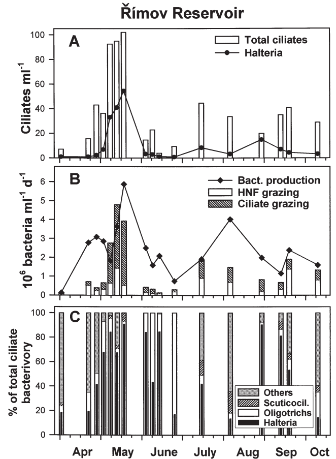
Fig. 2. The Římov Reservoir, April to October 1997. (A) Total ciliate abundance and abundance of Halteria , (B) bacterial production and total protistan bacterivory divided into heterotrophic flagellate (HNF) and ciliate grazing, and (C) the role of different ciliate taxa in total ciliate bacterivory. Note that the group 'oligotrichs' represents the aggregated bacterivory of all oligotrichous ciliates compared to the bacterivory of Halteria spp. only, and the group 'others' was dominated by grazing activity of peritrichous ciliates (for details see text)
