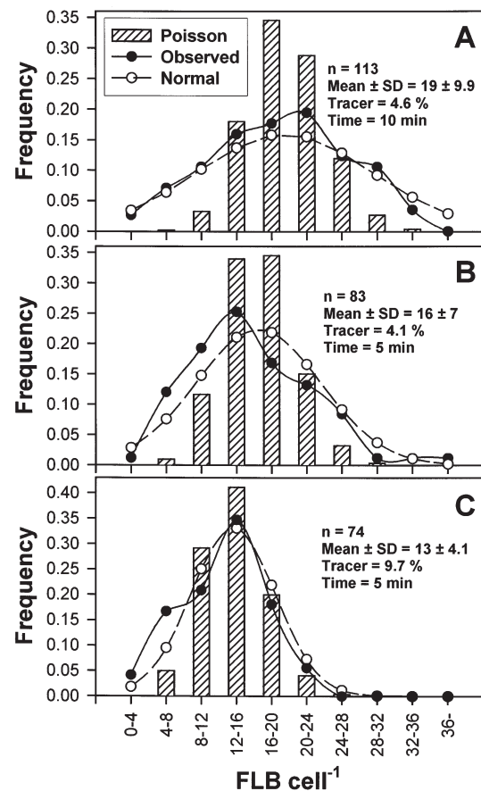
Fig. 1. Three examples of the frequency distribution of FLB uptake data of Halteria spp. representing samples with the highest abundance and number of ciliate individuals inspected. (A,B) The Sau Reservoir, 16 April 1997 and 10 July 1996, water temperature 16°C and 23.2°C, respectively; (C) The Římov Reservoir, 4 October 1994, water temperature 14°C. Each panel shows the corresponding parameters of mean uptake rate (fluorescently labelled bacteria [FLB] per cell \pm SD), number (n) of individuals inspected, tracer amount of FLB added, and time of incubation of the sample
