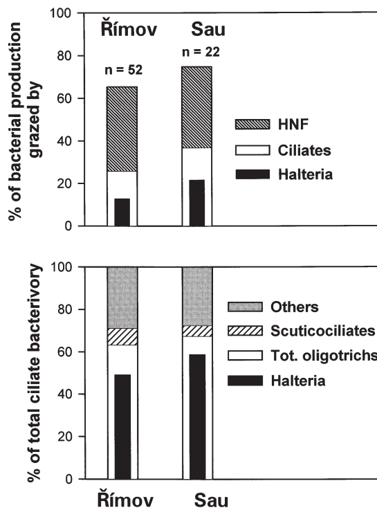
Fig. 4. (A) Overall averages (of n measurements) of the proportions of bacterial production grazed by all protozoans (the full size of the bars), grazed by HNF and ciliates separately, and grazed only by Halteria in the Římov (data from seasons 1993, 1994 and 1997) and Sau reservoirs (data from June 1996 to July 1997). (B) Overall averages of the role of different ciliate taxa in total ciliate bacterivory. For other explanations see Fig. 2
