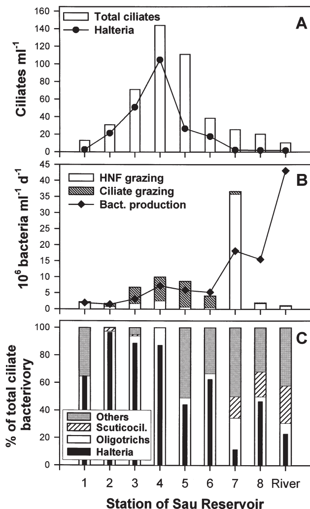
Fig. 3. An example of the longitudinal transects through the Sau reservoir, April 1997. (A) Total ciliate abundance and abundance of Halteria , (B) bacterial production and total protistan bacterivory divided into HNF and ciliate grazing, and (C) the role of different ciliate taxa in total ciliate bacterivory. For other explanations see Fig. 2
