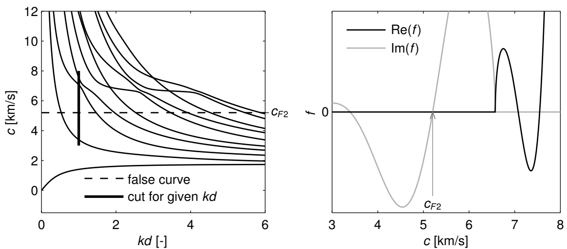
Fig. 9. The dispersion curves for antisymmetric modes and \phi = 45^\circ ; plot of function (7).
