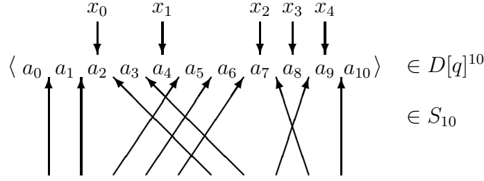
FIGURE 1. An element (a, \sigma) \in F_S(D[q])^{10} .
