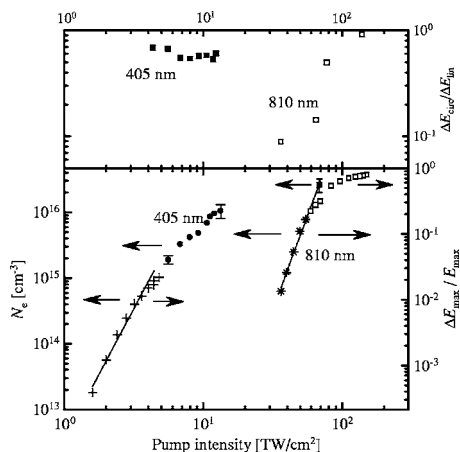
FIG. 4. Upper panel: measured ratio between the transient terahertz signal for circularly and linearly polarized pumps. Lower panel: Compilation of results showing the transient terahertz signal and free-electron density vs pump intensity for the linearly polarized pump. For low \Delta E_{\max} the transient wave forms scale with the pump intensity without significant reshaping. In this regime the free-electron density N_e is proportional to \Delta E_{\max} ; both vertical scales are relevant for such measurements (represented by the stars and crosses in the plot). For higher transient signal a significant reshaping of the transient terahertz wave form is observed: only one vertical scale then can be used for a given point as shown by the arrows (filled symbols: only left-hand scale is relevant; open symbols: only right-hand scale is relevant).
