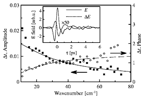
FIG. 6. Transient field transmittance \Delta t(\omega) at low pump intensity and the best fit using Drude model; pump wavelength: 405 nm; pump intensity: 3.2 \text{ TW/cm}^2 ; pump-probe delay: \tau_p=10 \text{ ps} . Inset: corresponding equilibrium E(\tau) and transient \Delta E(\tau, \tau_p) wave forms.
