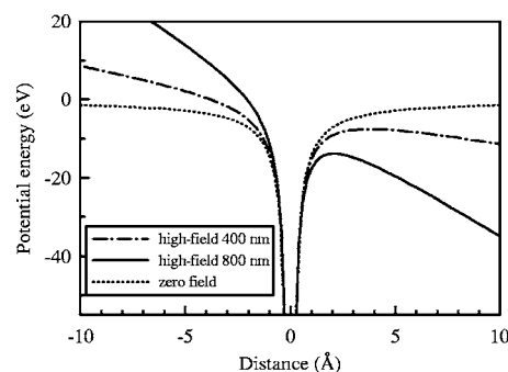
FIG. 3. Schematic picture of the influence of the laser electric field on the Coulomb potential due to the positively charged core felt by the electron in the static approximation. The maximum available values of the electric field for both experimental wavelengths were assumed in the plot.
