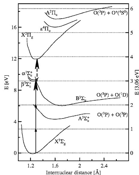
FIG. 2. Potential curves of \text{O}_2 and \text{O}_2^+ with the most probable multiphoton excitation and ionization process at 405 nm denoted by the arrows. The right-hand scale is normalized by the energy of 405-nm photons, i.e., it indicates the number of blue photons needed for a particular transition. The full arrow indicates the first resonant step and the dashed arrow indicates the second step involving the photoionization of the oxygen molecule.
