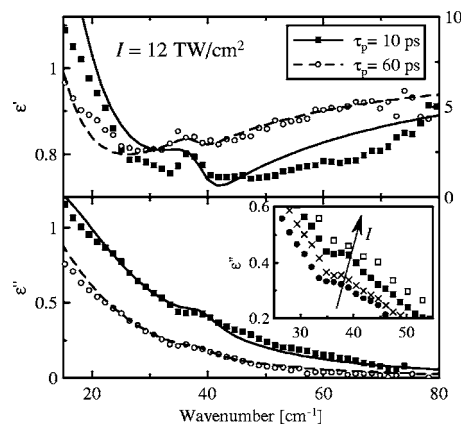
FIG. 8. Transient dielectric spectra obtained for I=12 \text{ TW/cm}^2 and two different pump-probe delays \tau_p=10 and 60 \text{ ps} and their fits using the Drude-Lorentz model (10) superposed with an underdamped harmonic oscillator at 39 \text{ cm}^{-1} ( \tau_p=10 \text{ ps} ) and at 38 \text{ cm}^{-1} ( \tau_p=60 \text{ ps} ). Inset: Imaginary part of the permittivity for several pump fluences ( 10.5 – 13.2 \text{ TW/cm}^2 ) at \tau_p=10 \text{ ps} .
