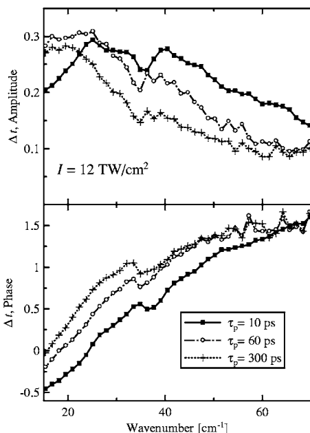
FIG. 9. Transient field transmittance spectra \Delta t(\omega) at I=12 \text{ TW/cm}^2 for the pump wavelength of 405 nm and for three significantly different pump-probe delays \tau_p .
