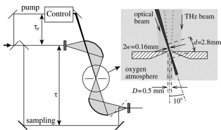
FIG. 1. Experimental scheme. The pump beam branch contains a specific arrangement for a careful control of the pump beam attenuation and polarization and a second-harmonic stage (see Appendix A for further details). Inset: detail of the geometry of the aperture and beams and of the interaction volume; d=D/\sin 10^\circ represents the length of the interaction region between the terahertz pulse and the plasma.
