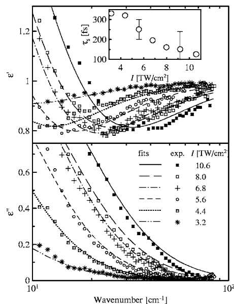
FIG. 7. Dielectric spectra of electronic plasma in photoionized oxygen calculated from transient wave forms using Eq. (3) and the fits by the Drude-Lorentz model (10) for several pump pulse intensities. Optical pump at 405 nm, linearly polarized, \tau_p=10 \text{ ps} . Inset: momentum relaxation time \tau_s extracted from the fits.
