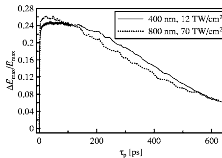
FIG. 5. Pump-probe scans: maximum field amplitude of the transient signal normalized by the maximum field amplitude of the reference wave form vs pump-probe delay.
