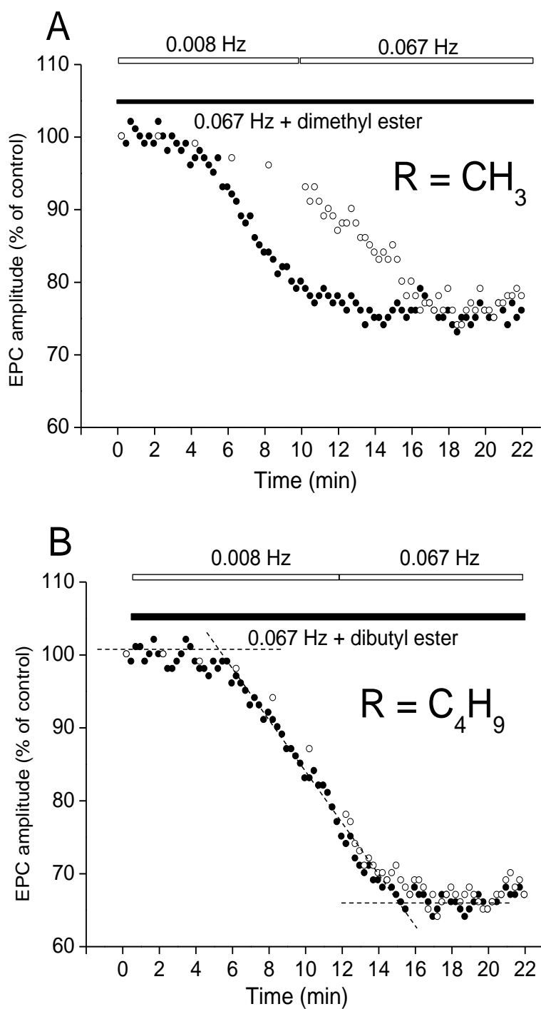
Fig. 2. A, Examples of effects of dimethyl ester ( 100 \mu\text{M} ), and B, dibutyl ester ( 100 \mu\text{M} ) on EPC amplitude in individual endplate. Results are expressed as percentage of the initial EPC amplitude during continuous higher frequency 0.067 \text{ Hz} stimulation (black circles, black bars). Open circles are EPC recordings which began during lower frequency stimulation ( 0.008 \text{ Hz} ) and continued during higher frequency ( 0.067 \text{ Hz} ) stimulation (open bars). EPC control amplitudes did not significantly differ in single experiments during both stimulation frequencies.
