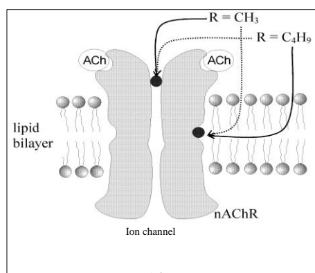
Fig. 4. Two possible action mechanisms of dimethyl and dibutyl ester.
