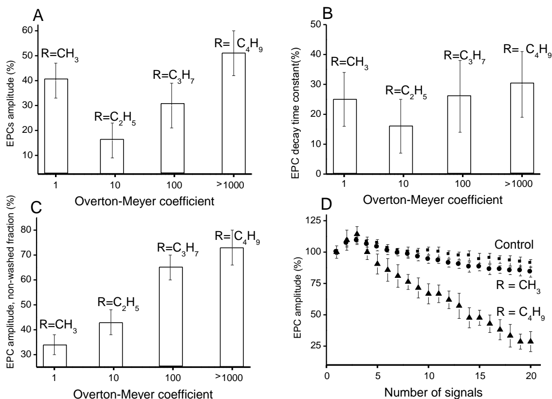
Fig. 3. EPC amplitude (A), decay time constant (B) and degree of drug washout (C, non-washed fraction of EPC amplitude inhibition as percentage of control amplitude) expressed as percentage of control values versus Overton-Meyer coefficients of the drugs (all applied at 500 \mu M concentration, n=5-10). Significantly different at probability level 0.05 were first and second columns on A and second and fourth columns on A, first and second vs. third and fourth columns on C. Decay times showed only tendency to change but mean values were not significantly different. For diethyl ester, \tau of fast decay component was presented. D, averaged series of EPC trains during high frequency stimulation (60 Hz) in controls (squares) before and after addition of 100 \mu M dimethyl- (circles) and 100 \mu M dibutyl- (triangles) esters.
