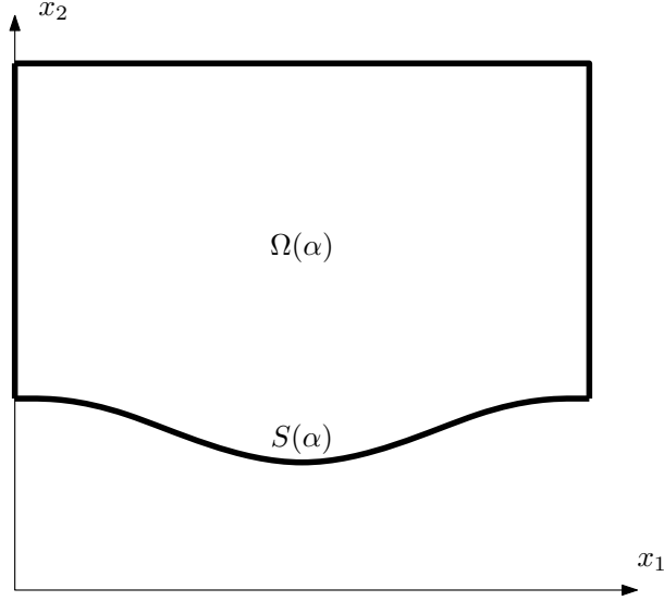
FIGURE 1. Geometry of the domain \Omega(\alpha) .
