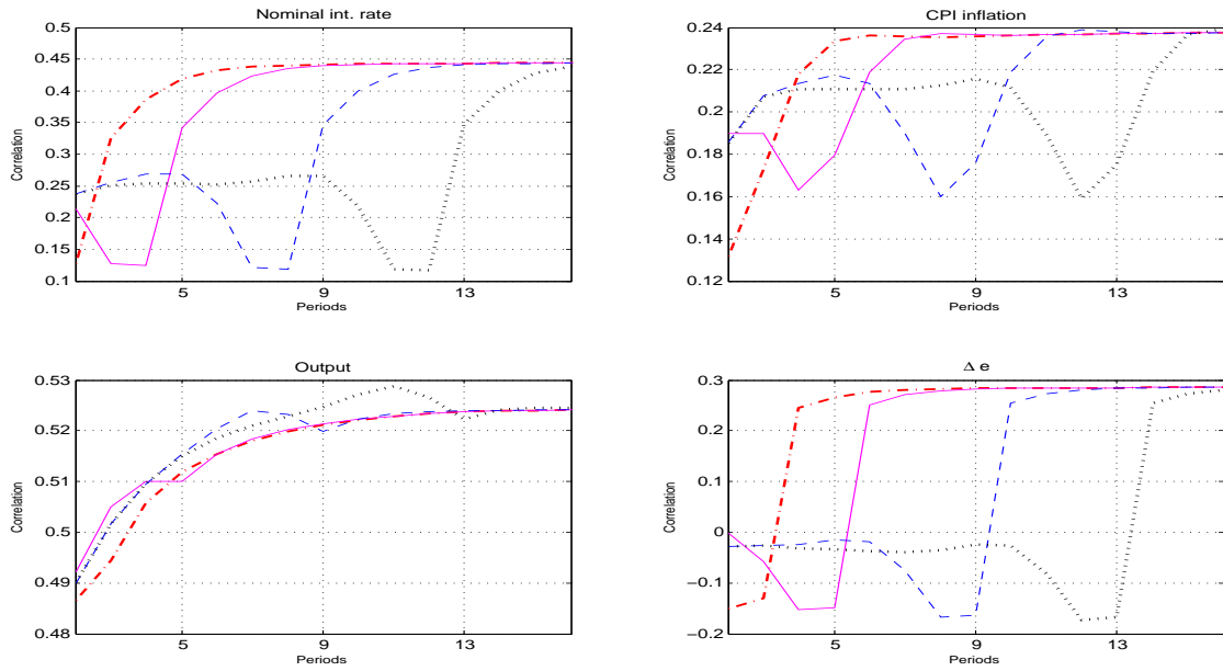
Figure 13: Correlation: y_t^*
