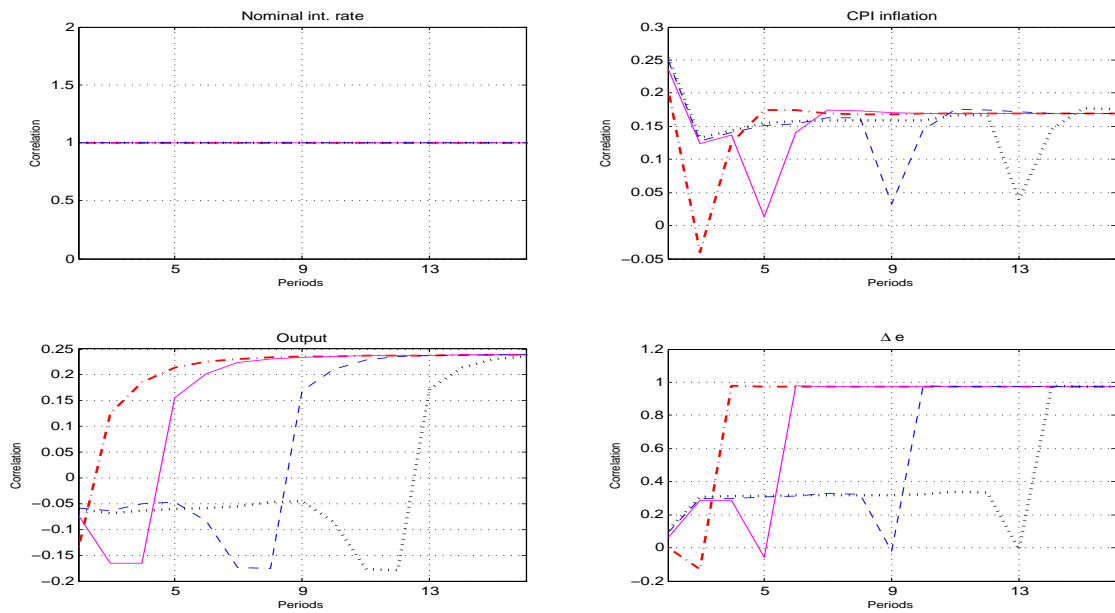
Figure 14: Correlation: i_t
