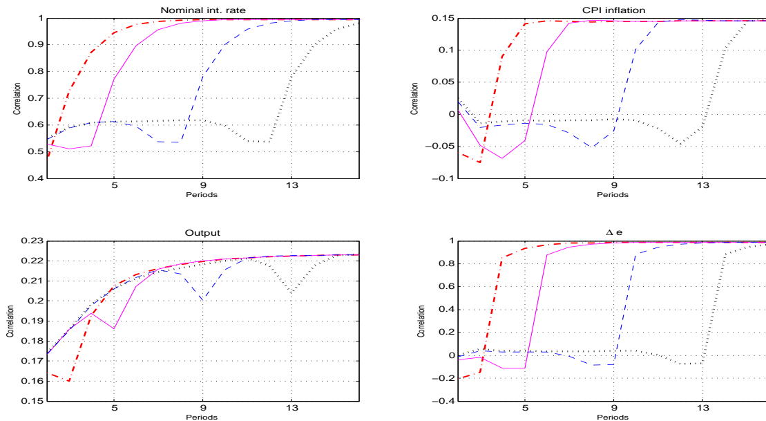
Figure 12: Correlation: i_t^*
