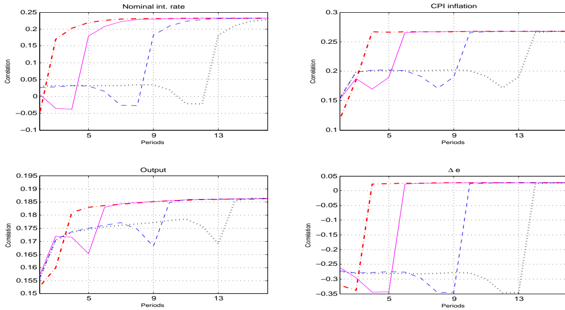
Figure 11: Correlation: \pi_t^*
