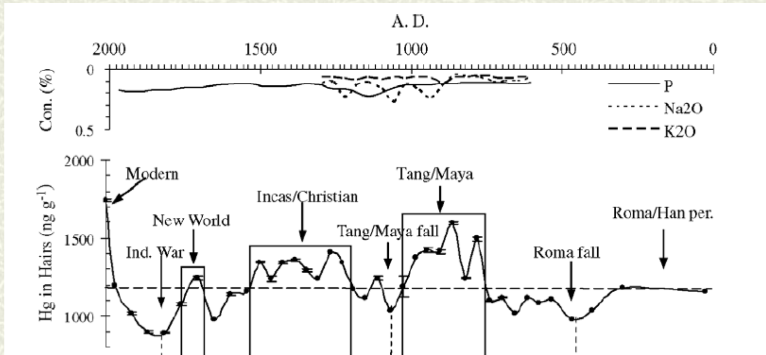
Fig. 2. (a) Concentrations of essential elements or compounds K 2 O (- - - -), Na 2 O (.....) and P (-) in the Antarctic seal hairs. (b) Hg T concentration in the Antarctic seal hairs. The parallel dash line represents the average concentrations of Hg T in the hairs. Known events about mercury consumptions
