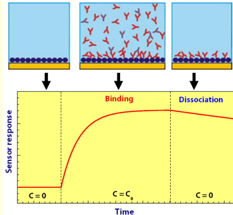
Typical SPR sensor response to (different stages of) molecular interaction occurring at the sensor surface.
